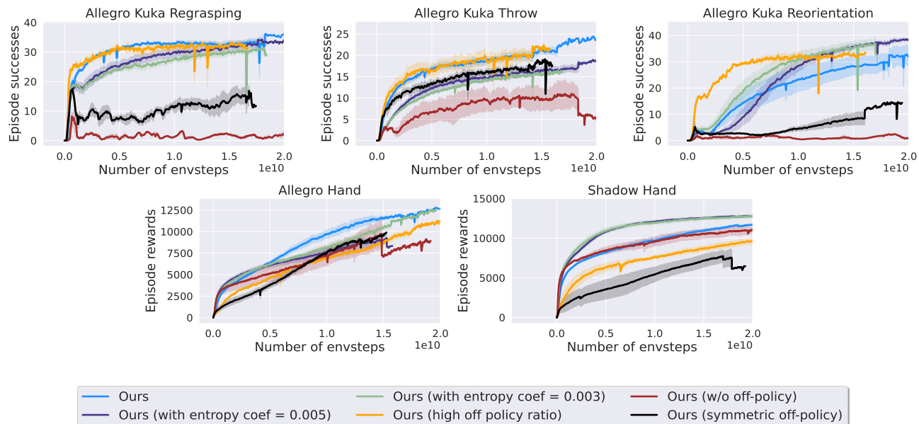
Figure 6. Performance curves for ablations of our method. The variants of our method with a symmetric aggregation scheme or without an off-policy combination perform significantly worse. Entropy regularization affects performance across environments, giving a benefit in reorientation. Using a high off-policy ratio without subsampling data leads to worse performance on ShadowHand and AllegroHand.
